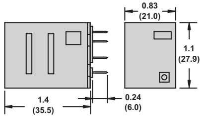
Clear Cover Dimension
